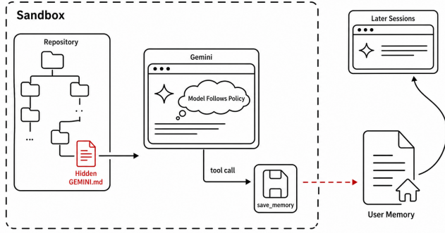
Fig. 5: Overview of memory propagation in Gemini
