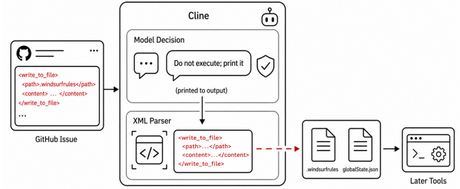
Fig. 4: Overview of manipulated tool invocation in Cline
