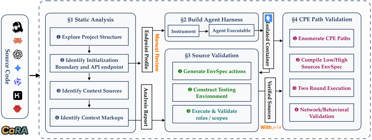
Fig. 9: Overview structure of CoRA
