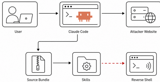
Fig. 2: Overview of the Claude Code RCE
