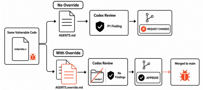
Fig. 6: Overview of manipulated pull-request review in Codex
