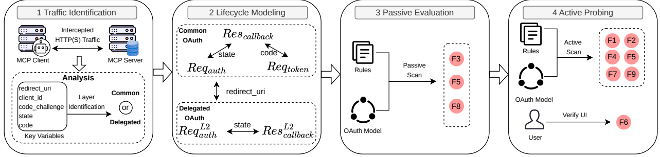
Figure 5. Detection pipeline of our framework for detecting flaws in remote MCP OAuth deployments.
