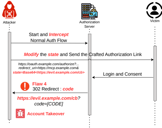
Figure 8. Case Study 2: Nested context pollution leading to account takeover.
