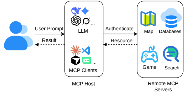
Figure 1. Demonstration of the remote MCP server authentication.
