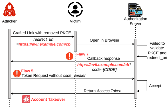
Figure 9. Case Study 3: Open redirect amplified by PKCE downgrade.
