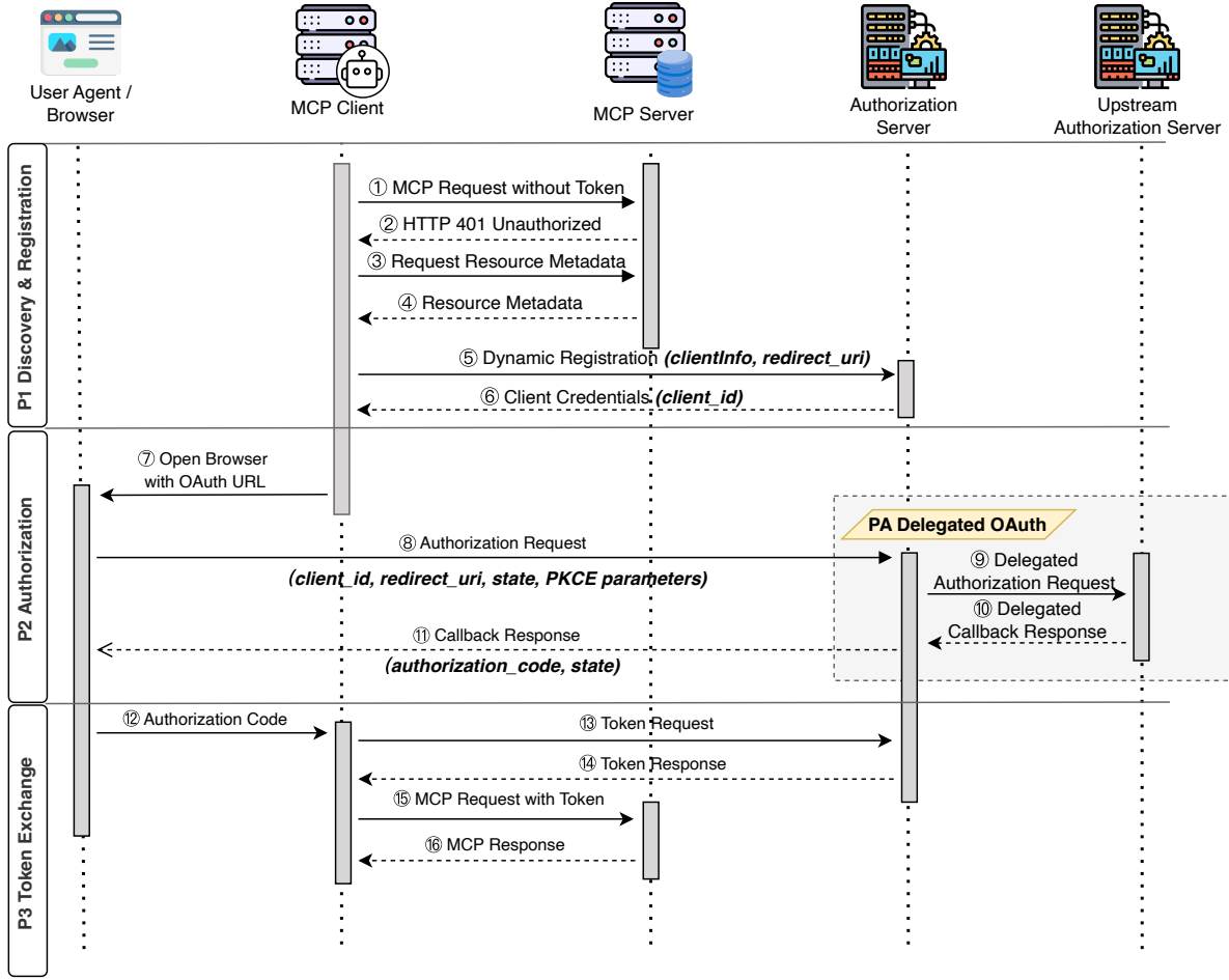
Figure 4. Workflow of OAuth-based authentication in remote MCP deployments. P1 - P3 capture the MCP client-to-server flow, while PA captures delegated authorization to upstream authorization services.
