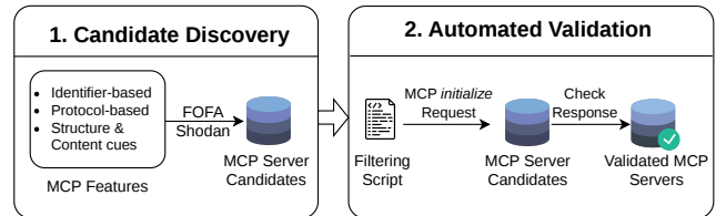
Figure 3. Two-step pipeline for discovering and validating remote MCP servers.
