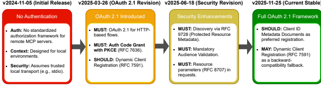
Figure 2. MCP specification authentication evolution timeline.
