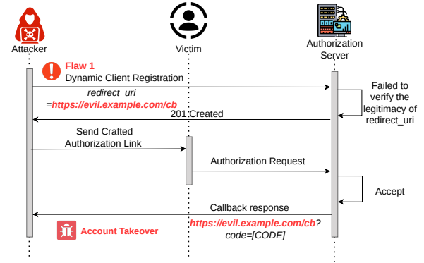
Figure 7. Case Study 1: Malicious client registration via open DCR.
