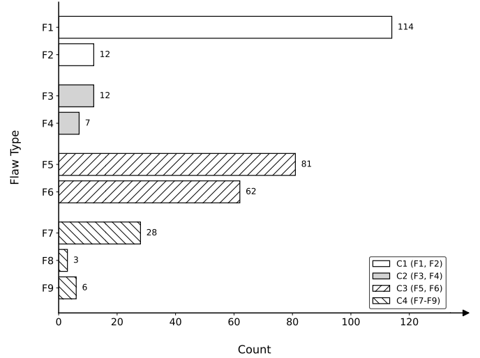
Figure 6. Overall flaw detection results on 119 MCP servers.
