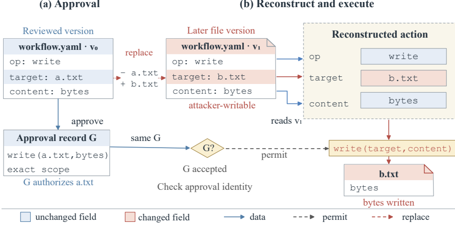
Fig. 1. Approval-to-execution divergence under post-review reconstruction. Grant G still authorizes write(a.txt) , but later mutable state reconstructs and executes write(b.txt) .
