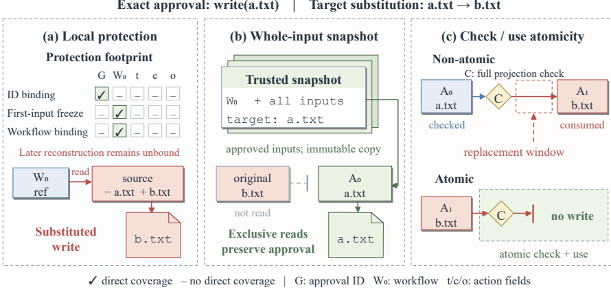
Fig. 5. Repair mechanisms and topology-dependent sufficiency. Local protection leaves reconstruction unbound; snapshot consumption and atomic check/use protect the object reaching the sink.
