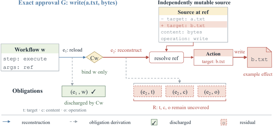
Fig. 4. Reconstruction path and authorization-obligation derivation. Binding the workflow at e_1 discharges (e_1, w) , but resolving an independently mutable source at e_2 leaves three residual obligations.
