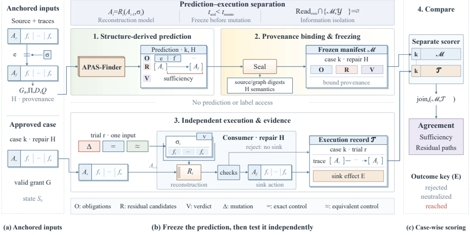
Fig. 3. Structure-derived prediction and independent execution validation. The executor does not read frozen predictions or labels; a separate scorer compares them with final sink effects.
