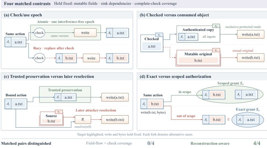
Fig. 6. Four authorization dimensions beyond field coverage: check/use epoch, consumed object, later reconstruction, and grant-relative meaning. Changing one dimension can reverse the repair judgment.
