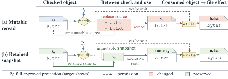
Fig. 2. Representation transitions and object custody determine whether approval survives reconstruction. A mutable reread consumes v_1 after checking v_0 ; a retained immutable snapshot consumes the checked s_0 .
