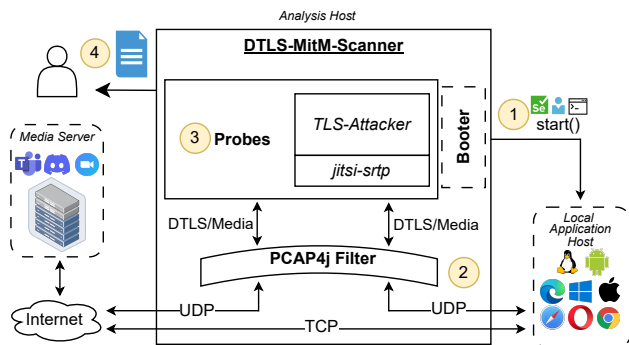
Figure 2: Sketch of the DMS architecture.
