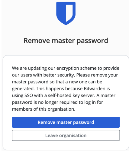
Figure 3: Key Connector conversion page with malicious message injected by the adversary.
