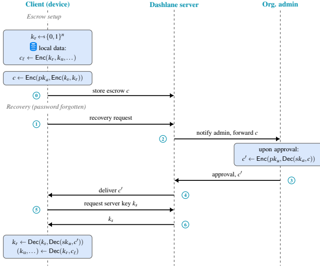
Figure 4: Dashlane’s admin-assisted key escrow and recovery flow. During setup, the client stores the local data encrypted under the recovery key k_r (which never leaves the device), and uploads the escrowed recovery key c (step 0), wrapped first under a server-provided symmetric key k_s and then under the admin public key pk_a . To recover (1), the server forwards c to the admin (2); the admin peels off the RSA-OAEP layer and re-encrypts to the user (3, 4), after which the client retrieves k_s from the server (5, 6) and unwraps k_r .
