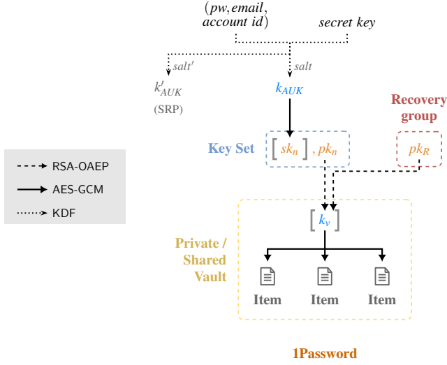
Figure 2: Key hierarchy for 1Password. Some levels of key wrapping have been omitted for simplicity. For instance, k_{AUK} encrypts the symmetric key in the key set, which in turn encrypts the secret key—here we show the k_{AUK} as directly encrypting sk_n .
