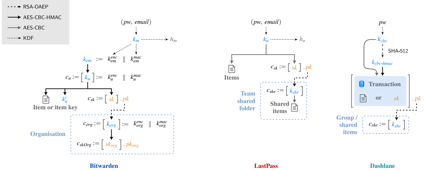
Figure 1: Key hierarchies for Bitwarden (left), LastPass (centre) and Dashlane (right).
