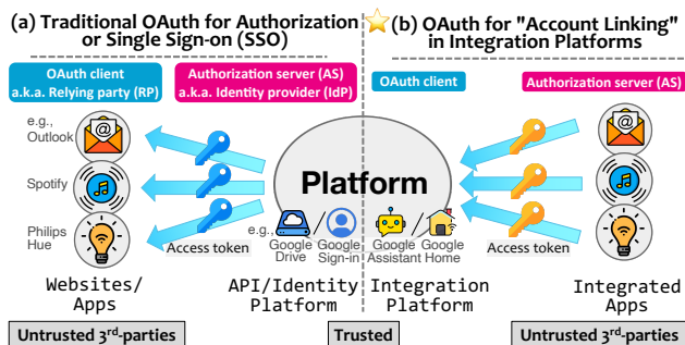
Figure 3: Flipped Paradigm: OAuth Role Reversal
