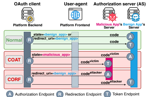
Figure 4: Insufficiency in Active App Tracking
