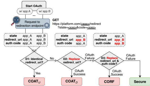
Figure 9: Decision Tree for Vulnerability Detection
