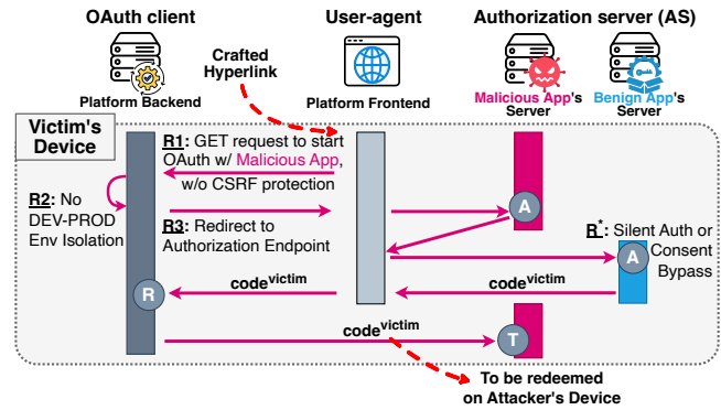
Figure 6: Worst-case Scenario: Single-click COAT Attack without Malicious App Distribution
