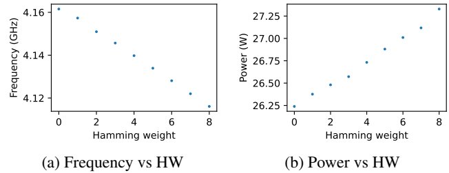
Figure 6: Effect of varying the number of non-consecutive 1s in the \text{LEFT} = \text{RIGHT} input to Figure 3b’s sender on our i7-9700 CPU. The results confirm that larger HWs cause higher power consumptions and lower steady-state frequencies.
