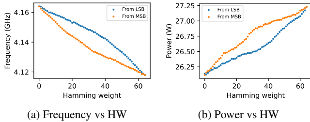
Figure 5: Effect of varying the number of consecutive 1s in the \text{LEFT} = \text{RIGHT} input to Figure 3b’s sender on our i7-9700 CPU. As we increase the number of 1s, the mean power consumption grows and the mean steady-state frequency drops.
