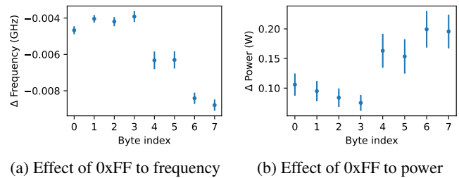
Figure 7: Effect of setting single bytes to 0xff in the \text{LEFT} = \text{RIGHT} input to Figure 3b’s sender on our i7-9700 CPU. The effect varies depending on the position of 1s within the inputs. HW differences in the MSBs have the strongest effect; HW differences in the bits right below 32 have the weakest effect.
