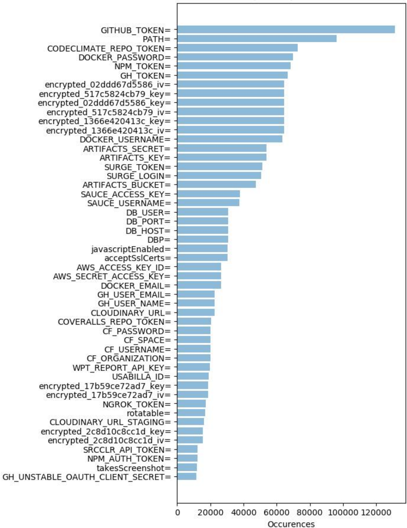
Most common [secure] variables on Travis CI
