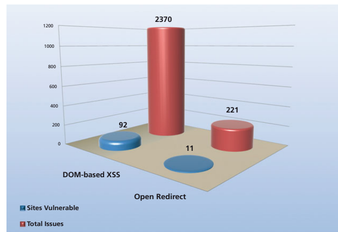
Figure 3: Distribution of vulnerability types (DOM-based Cross-site Scripting vs. Open redirects)
